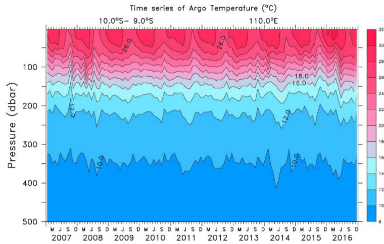
Gambar 7. Profil Upwelling dan downwelling dari permukaan laut hingga kedalaman 500 m. Figure 7. Upwelling and downwelling profile from surface to 500 m depth.
