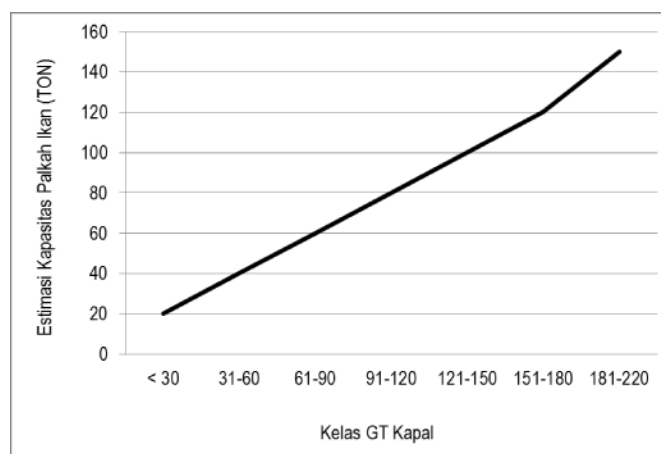
Gambar 3. Estimasi kapasitas palkah ikan pada kapal pukat cincin yang didaftarkan DJPT ke WCPFC. Figure 3. Estimation of fish-hold capacity of the large pelagic purse seiners that are registered by DGCF to WCPFC.
