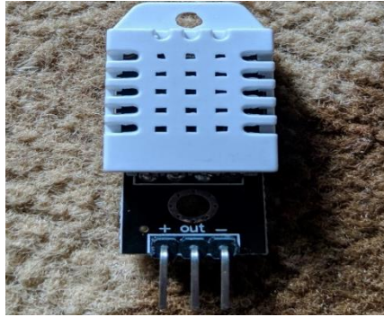
Gambar 2. Sensor DHT 22
